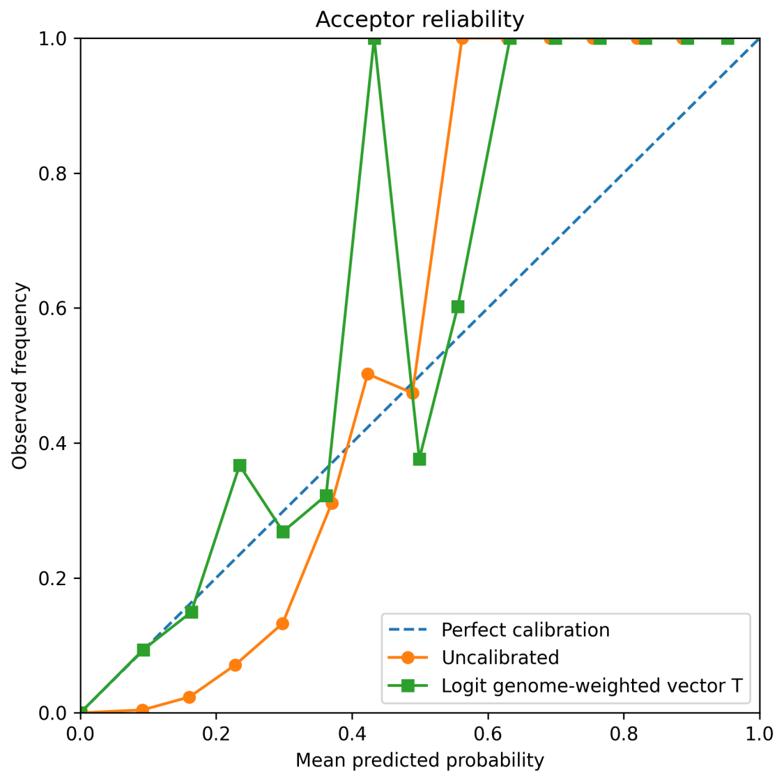
Figure 3C. Acceptor reliability before and after calibration.
