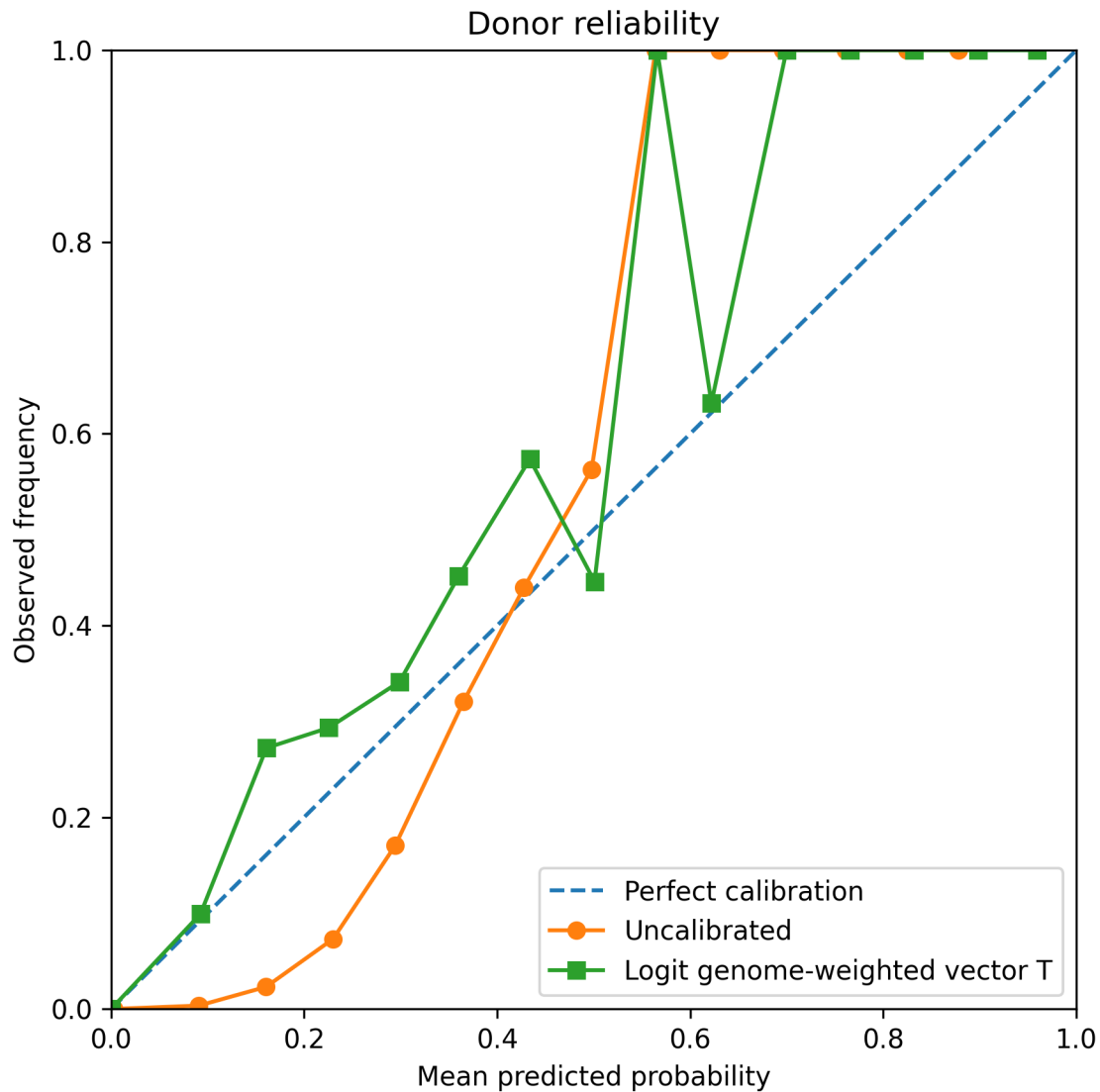
Figure 3D. Donor reliability before and after calibration.
