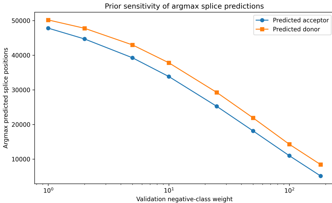
Figure 5C. Prior sensitivity of argmax prediction counts.
