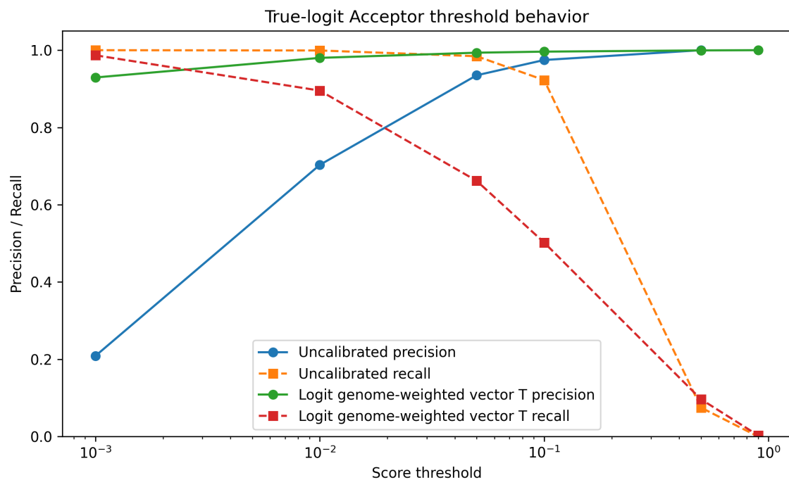
Figure 4A. Acceptor threshold precision-recall behavior.
