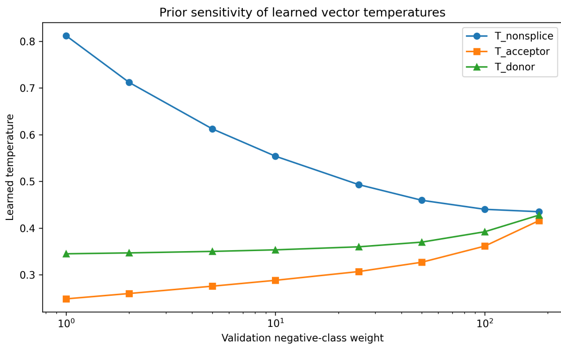
Figure 5A. Prior sensitivity of learned temperatures.
