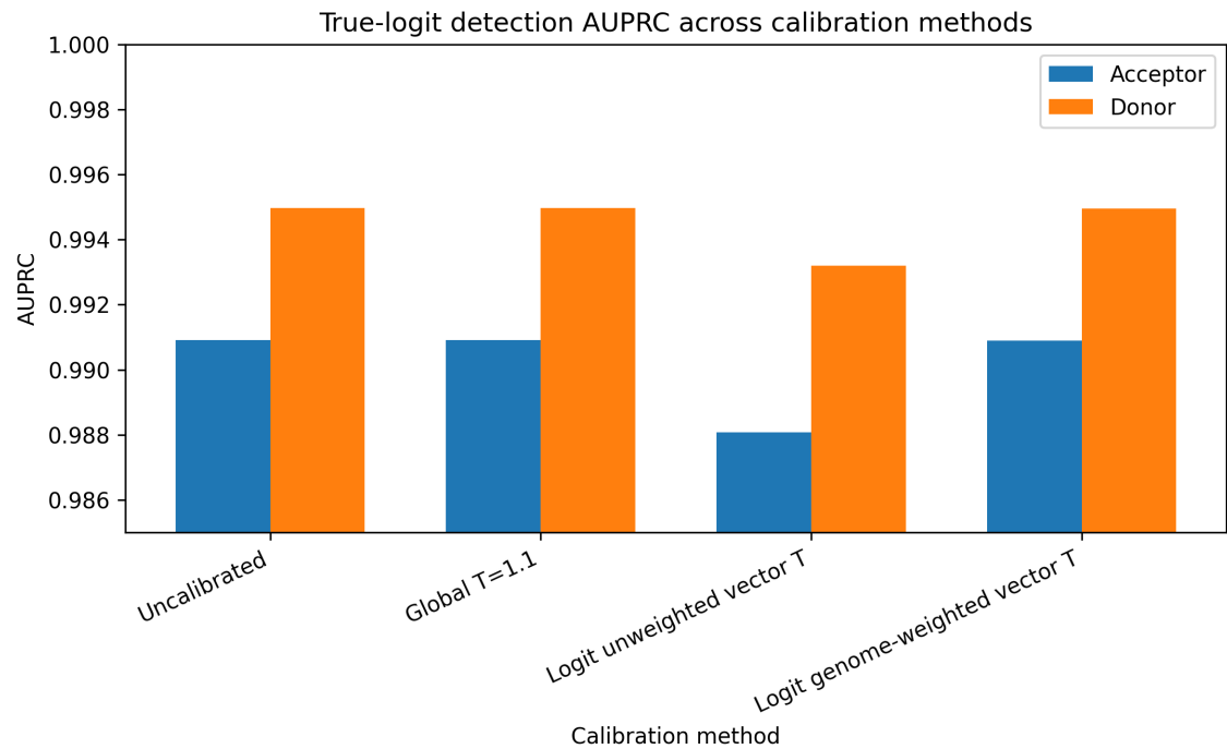
Figure 2. Acceptor and donor AUPRC across calibration methods.
