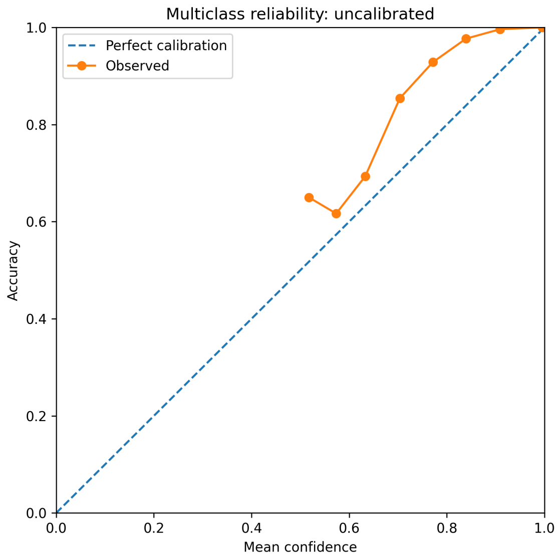
Figure 3A. Multiclass reliability before calibration.
