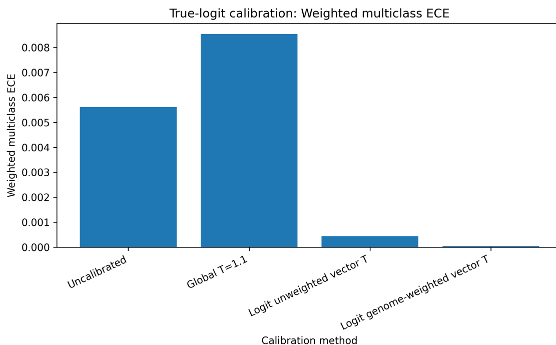
Figure 1A. Weighted multiclass expected calibration error.
