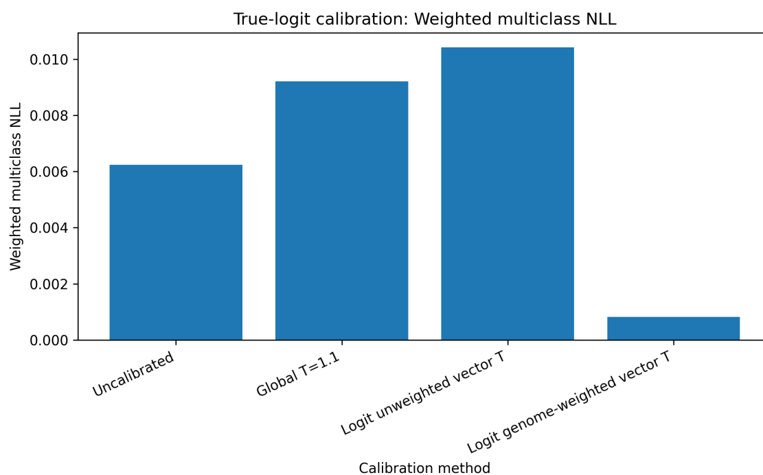
Figure 1B. Weighted multiclass negative log-likelihood.
