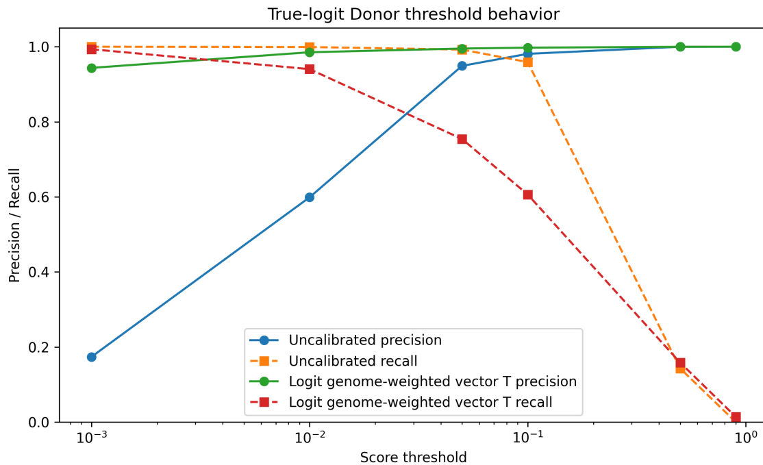
Figure 4B. Donor threshold precision-recall behavior.
