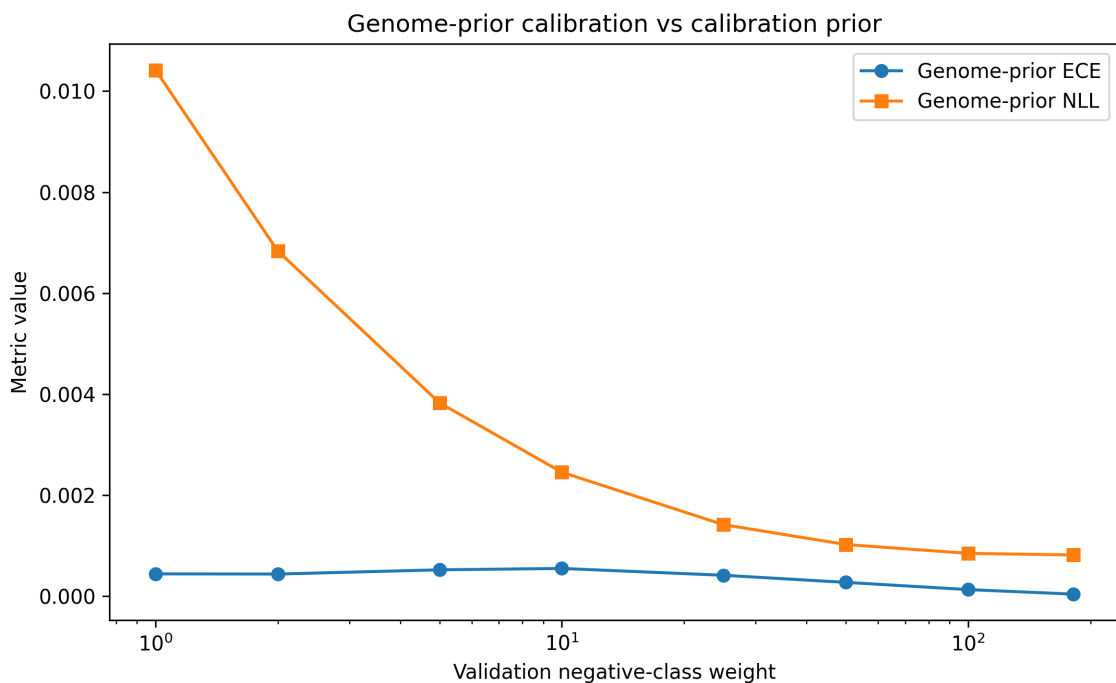
Figure 5B. Prior sensitivity of genome-prior calibration metrics.
