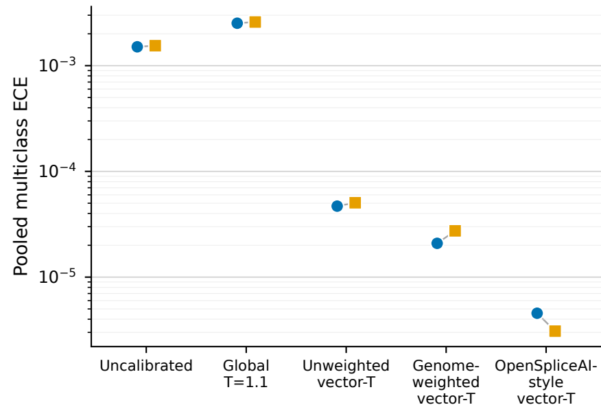
(a) Expected calibration error
