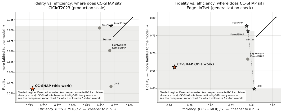
Figure 2: Fidelity–Efficiency Frontier, CICIoT2023 (left) and Edge-IIoTset (right).
