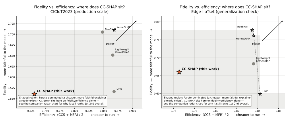
Figure 2. Fidelity–Efficiency Frontier, CICIOT2023 (left) and Edge-IIoTset (right).
