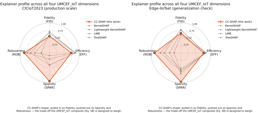
Figure 4. Radar-chart explainer profiles, CICIoT2023 (left) and Edge-IIoTset (right).
