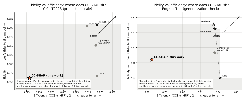
Figure 2. Fidelity–Efficiency Frontier, CICIoT2023 (left) and Edge-IIoTset (right).
