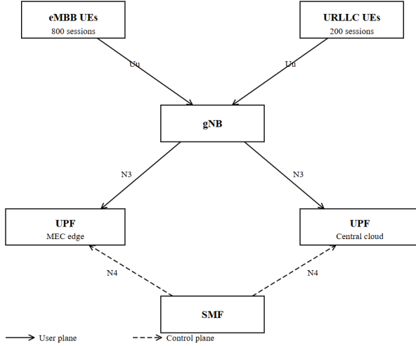
Fig. 1. 5G multi-UPF network architecture. eMBB and URLLC UEs connect to the gNB via the Uu air interface. The gNB forwards traffic over N3 to either the MEC edge UPF or the central cloud UPF. The SMF steers sessions between both UPFs via the N4 control interface.
