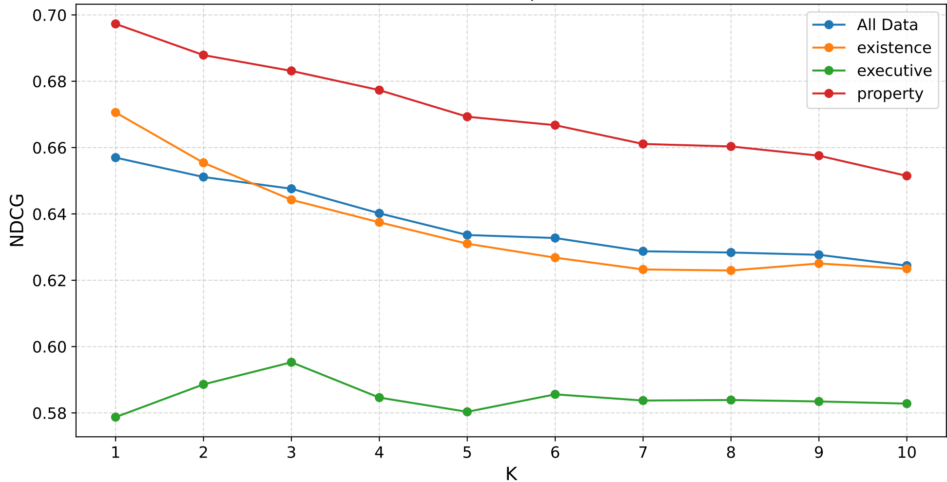
NDCG Line Graph across K
