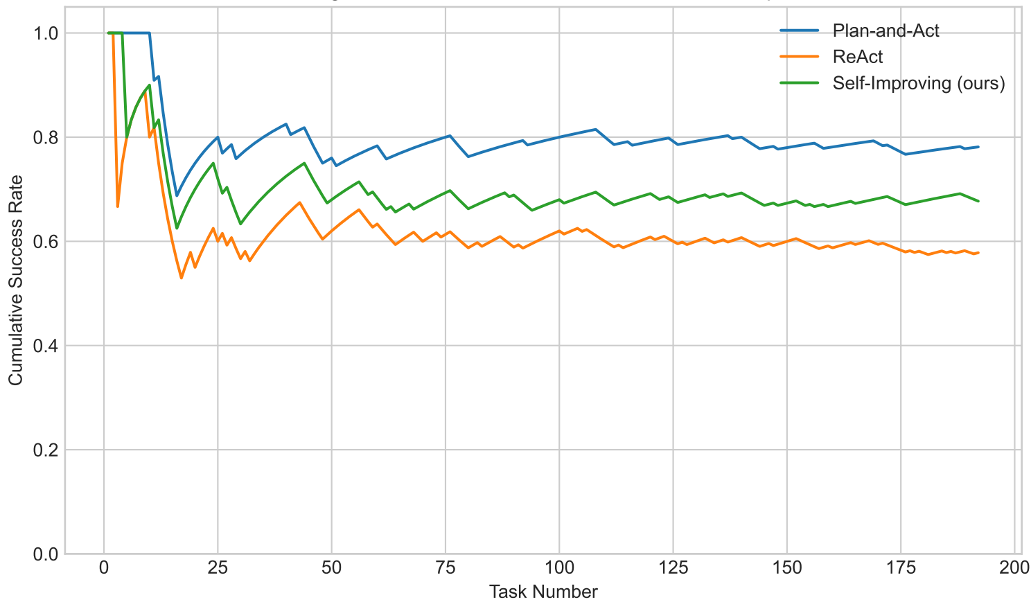
Learning Curve: Cumulative Success Over Task Sequence
