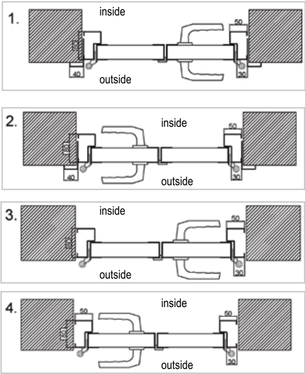
Side Hinged Garage Door fitting and opening option
