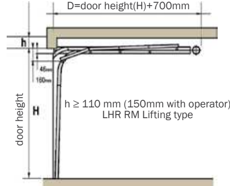
LHR RM low headroom lift double tracks, rear mounted springs
