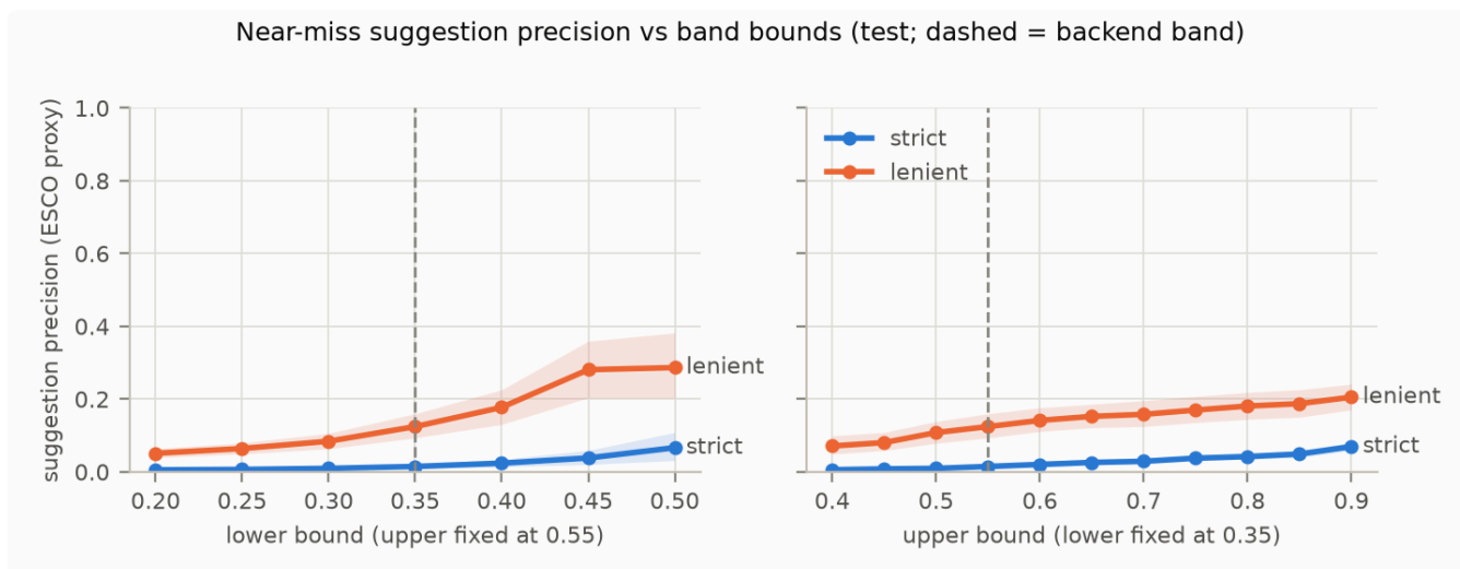
Figure 9. Test precision as one bound of the old band moves and the other stays fixed (dashed line = the old app's value). Raising either bound improves precision; shaded areas are 95% intervals.
