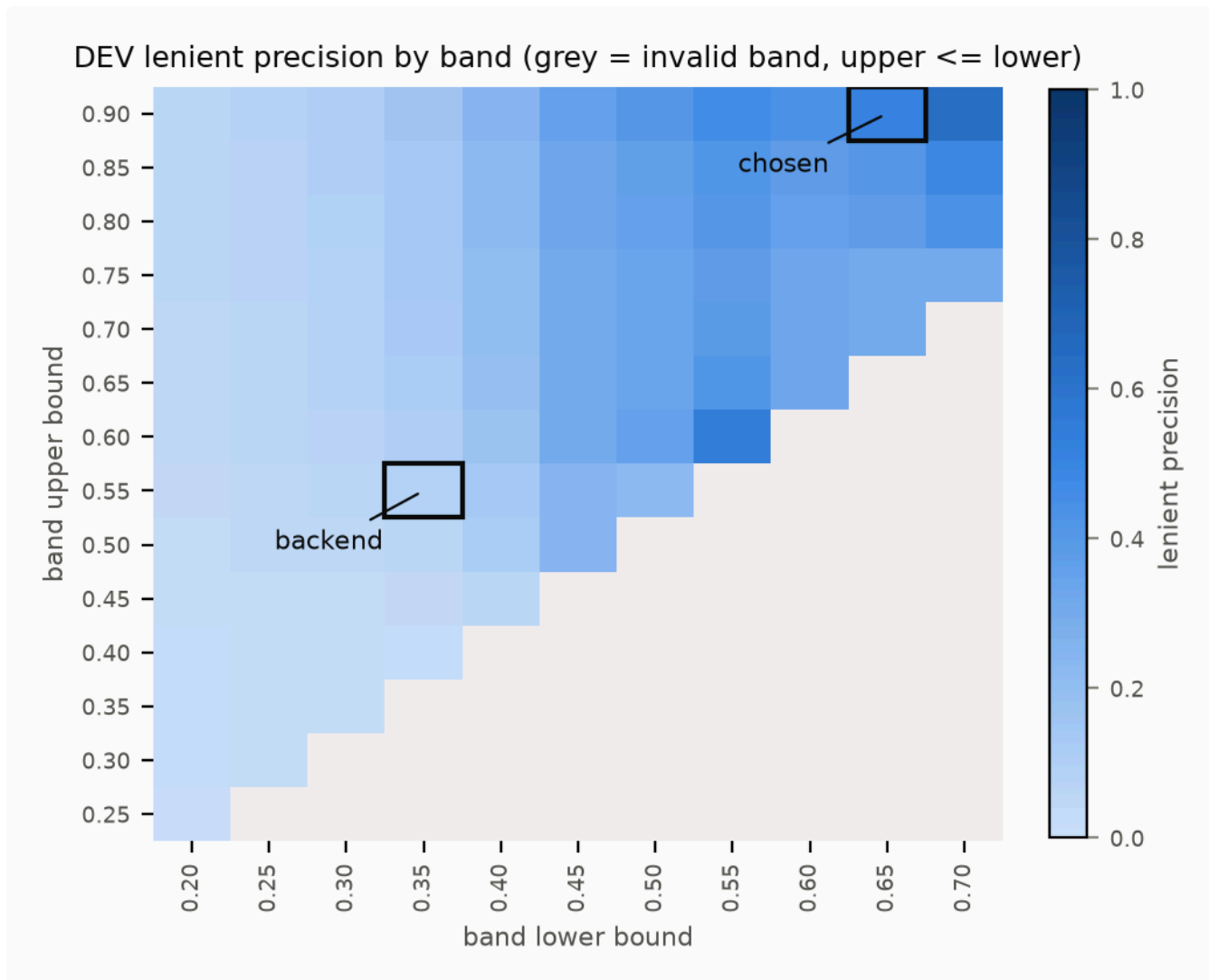
Figure 8. Dev precision of every band. Precision rises with the lower bound; bands below 0.5 are near the base rate.
