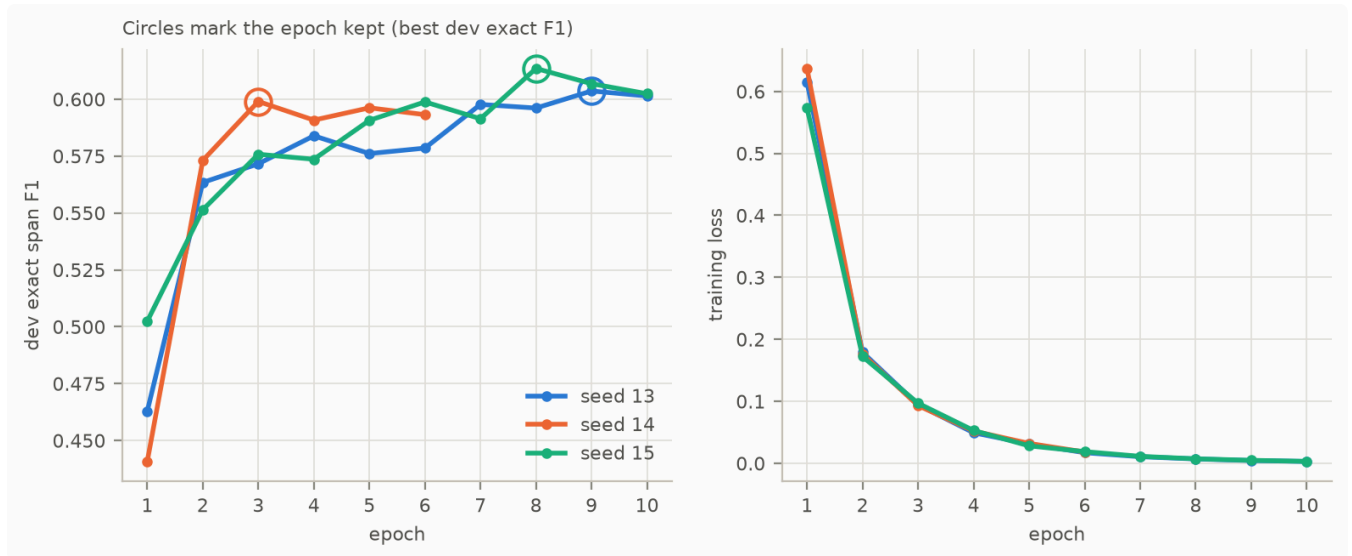
Figure 3. Training curves. Loss falls from about 0.6 to near zero within ten epochs; dev F1 plateaus near 0.60 after epoch 3. Seed 14 stopped early at epoch 6.
