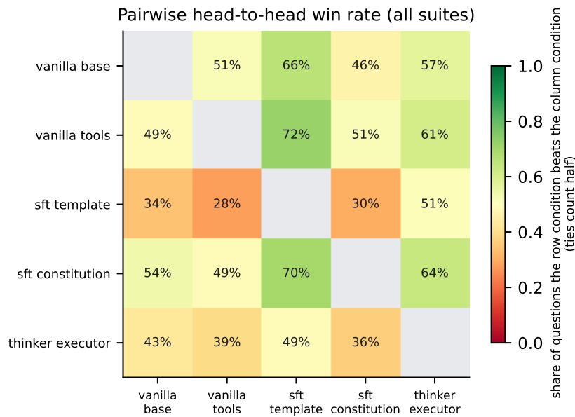
Figure 5.13: Win rate for every pair of conditions on the questions both answered. Each cell reads as the row condition’s share of contests won against the column condition, so the matrix is symmetric about 0.5.
