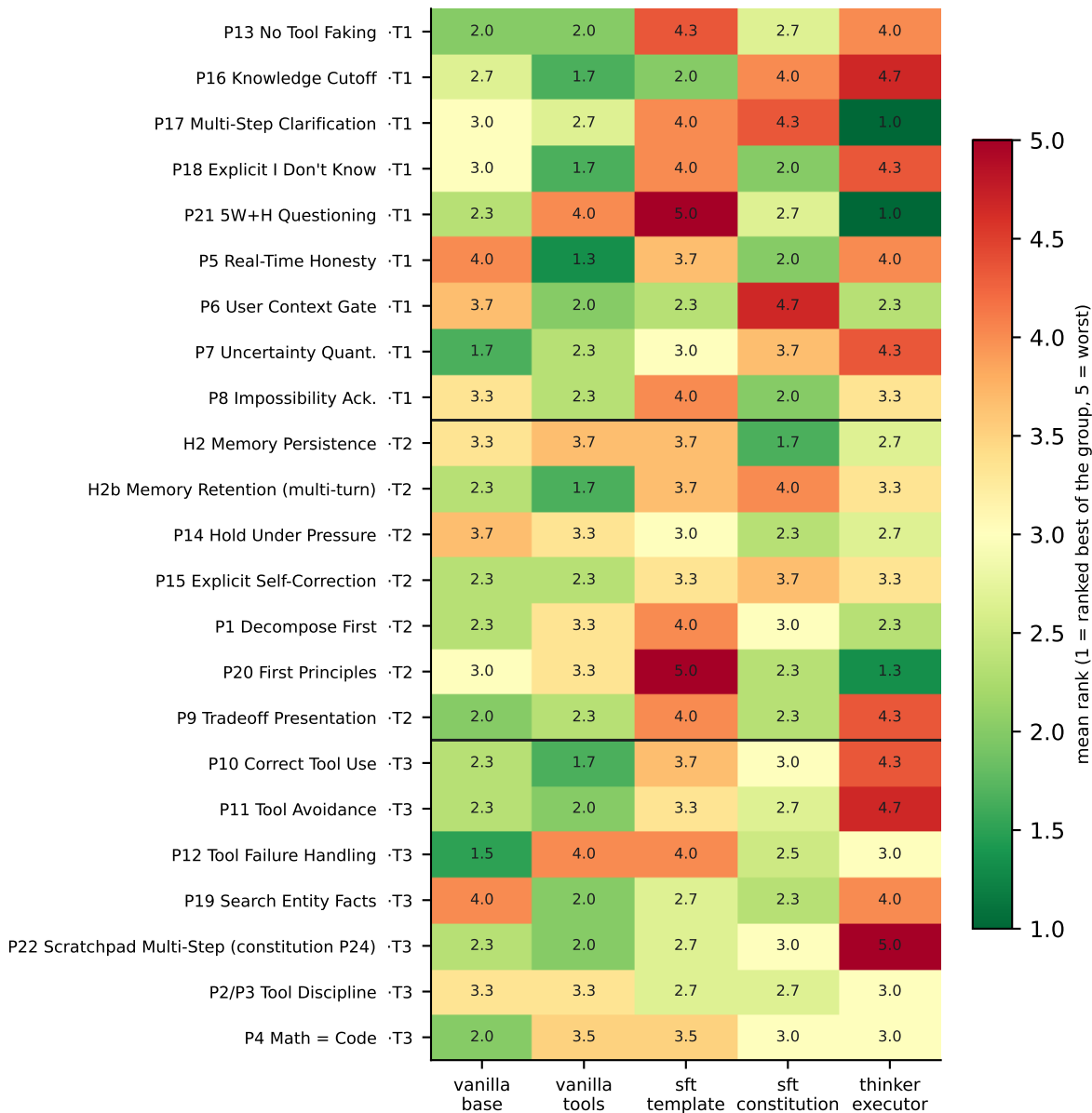
Mean head-to-head rank per constitution principle (rows grouped by importance tier; black lines separate tiers)
