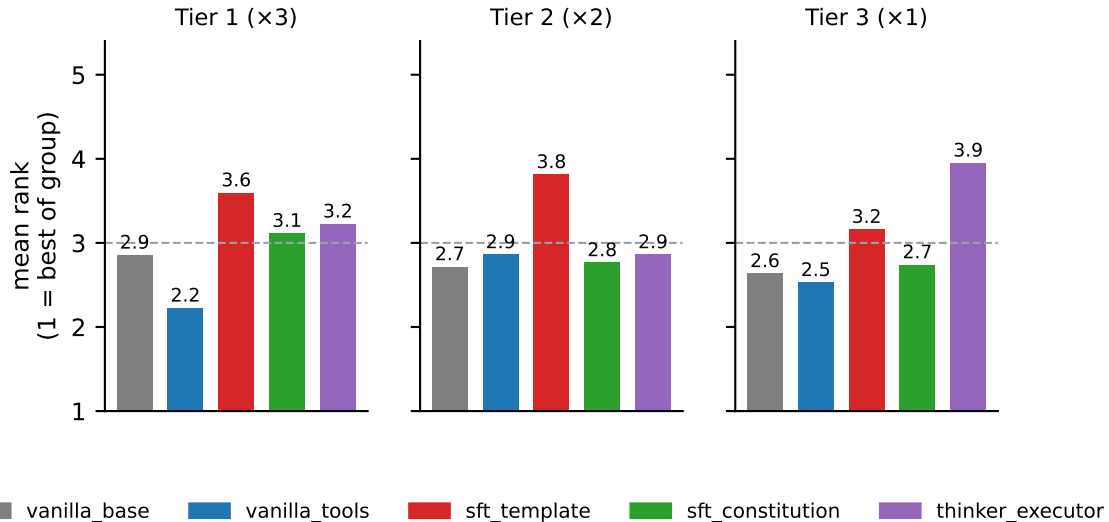
Mean rank by principle importance tier — constitution suite
