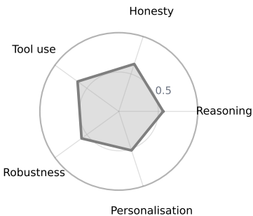
vanilla base
