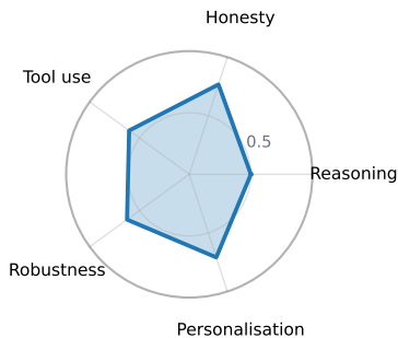
vanilla tools
