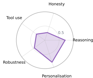
thinker executor
