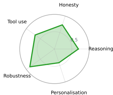
sft constitution
