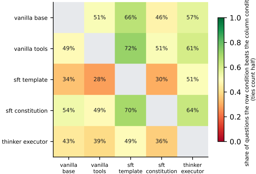
Pairwise head-to-head win rate (all suites)
