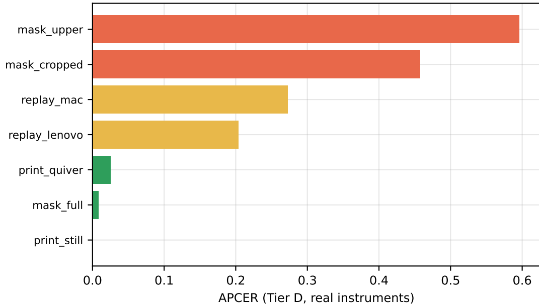
(b) works when eyes are occluded, fails when real eyes are present
