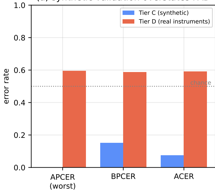
(a) synthetic validation overstates PAD
