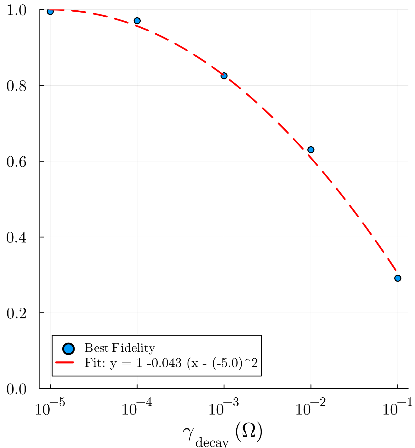
Best Fidelity
