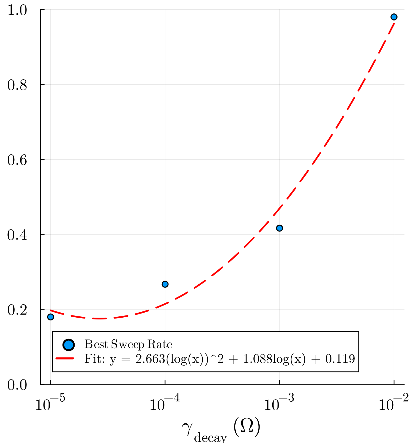
Best Sweep Rate ( \Omega^2 )
