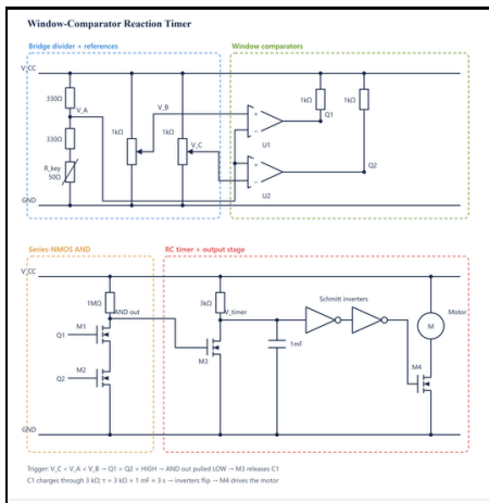
FIG. 3: Schematic: Wheatstone bridge, dual comparator, NMOS AND, RC Timer
