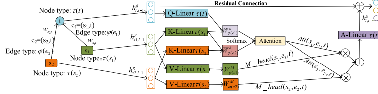
Fig. 8. Log heterogeneous graph representation based on HG2N.
