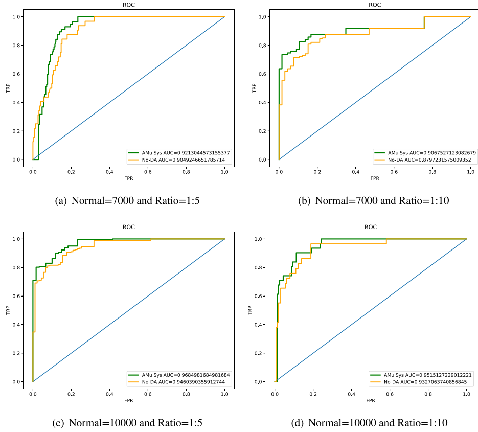
Fig. 11. ROC curve under imbalanced data.
