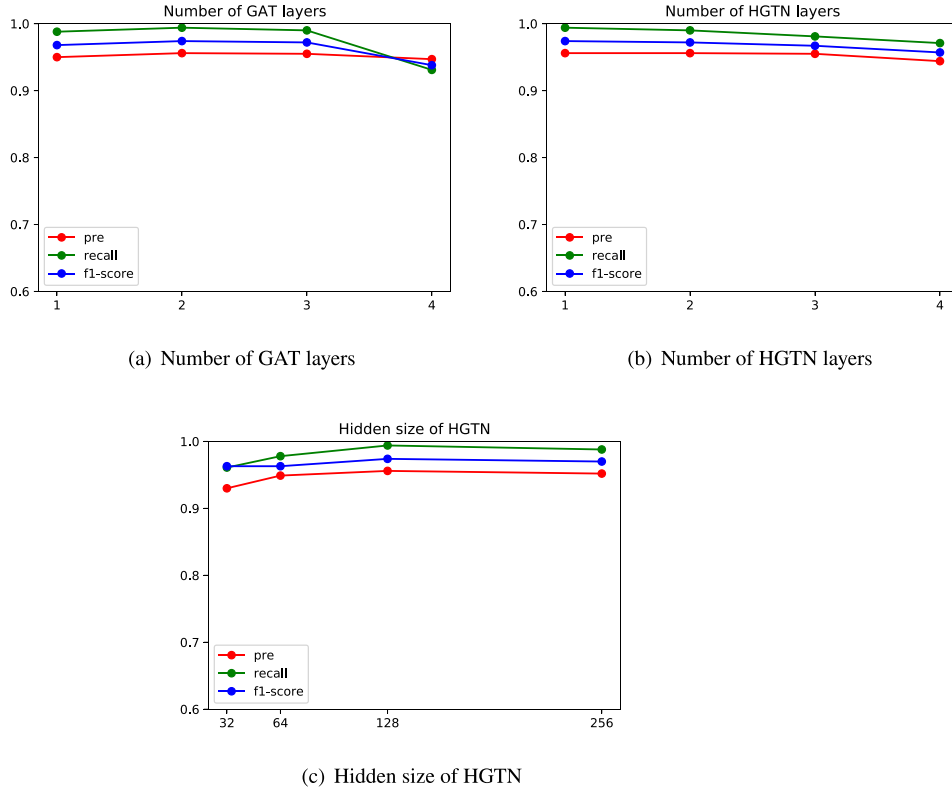
Fig. 9. Anomaly detection results for different parameters.
