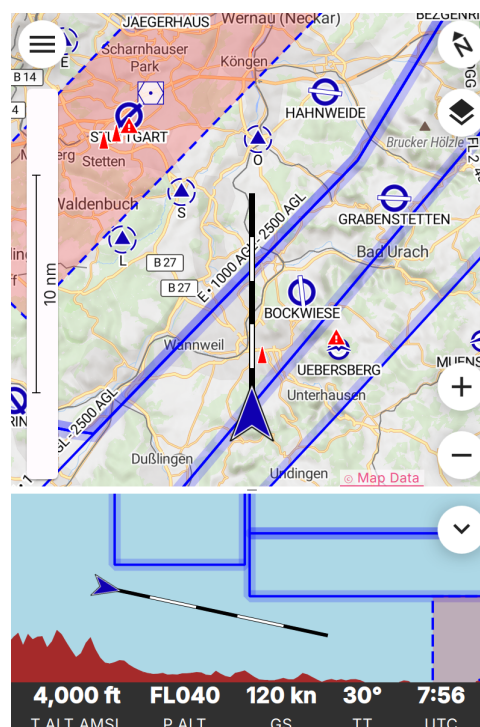
Fig. 5: Side View of the Airspace while Approaching EDDS
