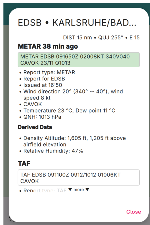
Fig. 2: METAR and TAF Dialog
