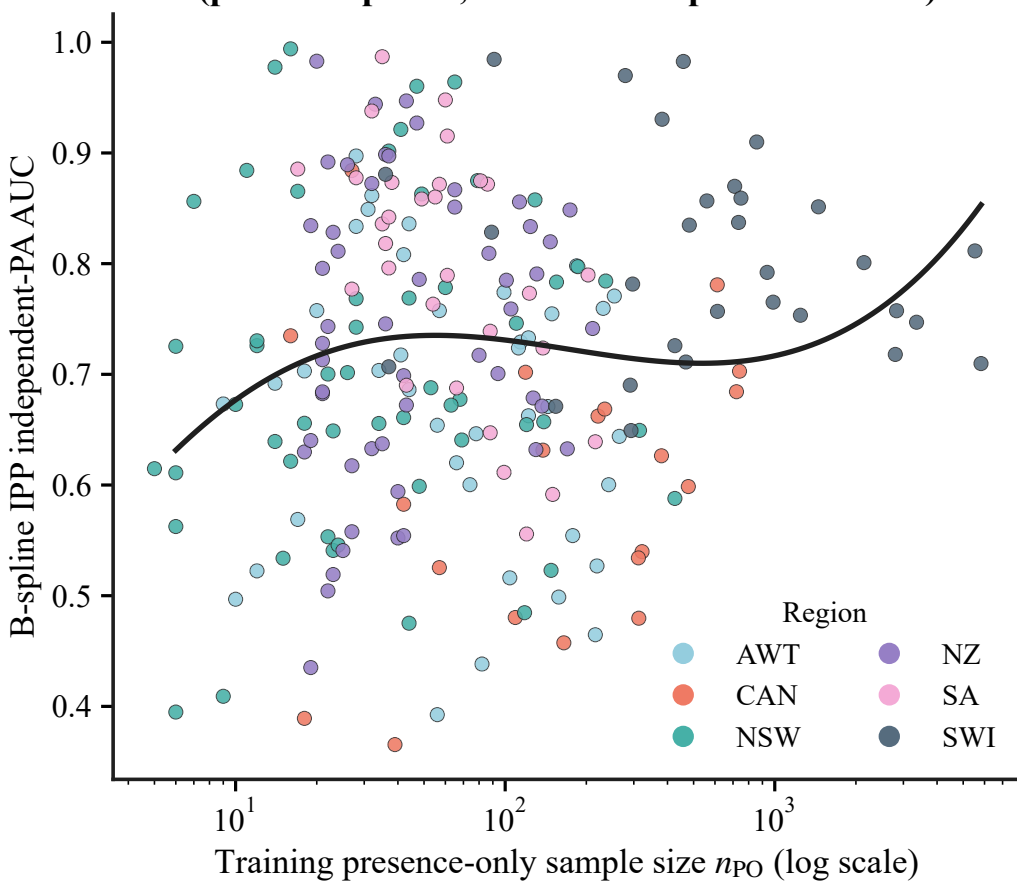
C B-spline IPP AUC versus training sample size (points = species; black line = spline smoother)
