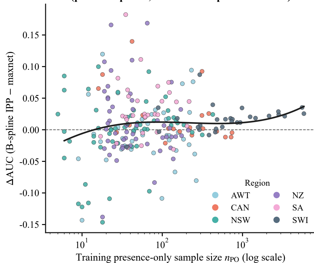
D \Delta AUC (B-spline IPP – maxnet) versus sample size (points = species; black line = spline smoother)
