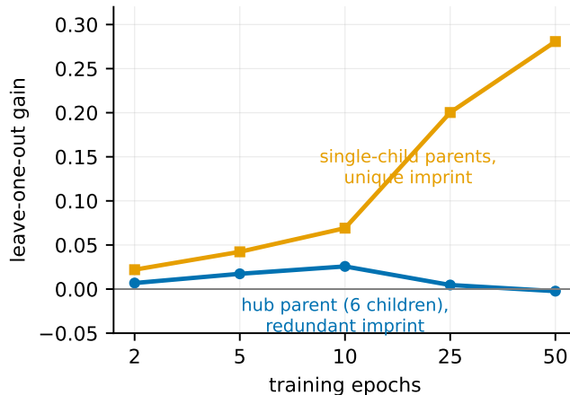
Figure 1: Maturity collapse is redundancy-ordered, not uniform. Leave-one-out gain versus training epochs on a hub-structured synthetic network (mean of two system seeds). Gains for the hub parent, whose imprint is redundant across six children, rise, peak at partial maturity, and collapse to zero as the model learns alternative routes; gains for single-child parents, whose imprint is unique, grow monotonically. Uniform degradation—the overfitting signature—is absent.
