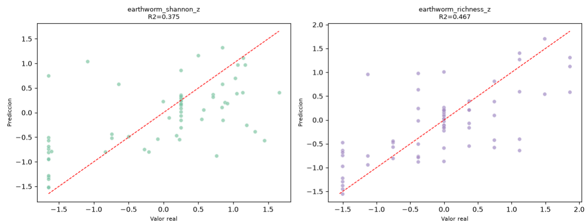
Prediccion vs Valor Real - MLP Custom Loss (eval.csv)
