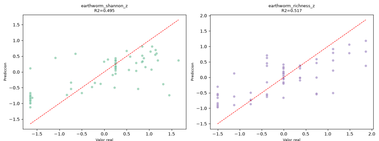
Prediccion vs Valor Real - XGBoost (eval.csv)
