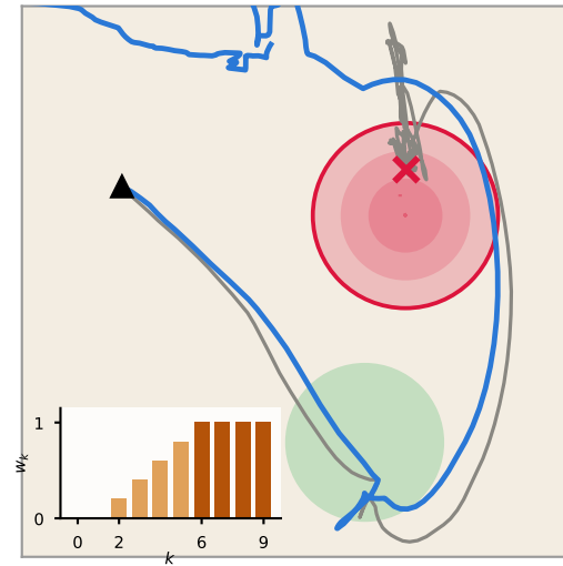
(c) Enforce: executed paths, ours vs base (inset: repair weight w_k per Euler step)
