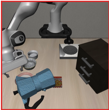
(a) unshielded policy: drives through the hazard --- moka pot toppled
