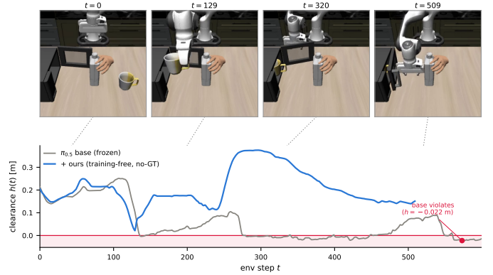
Fig. 6. The certificate at work over one episode (the pair of Fig. 1). Clearance h(t) to the hand-attached hazard: the unfiltered base policy (gray) crosses h=0 at t=136 and spends 215 of 600 steps in violation; ours (blue) dips to +0.021 m at its closest approach and never crosses, completing the task at t=510 .
