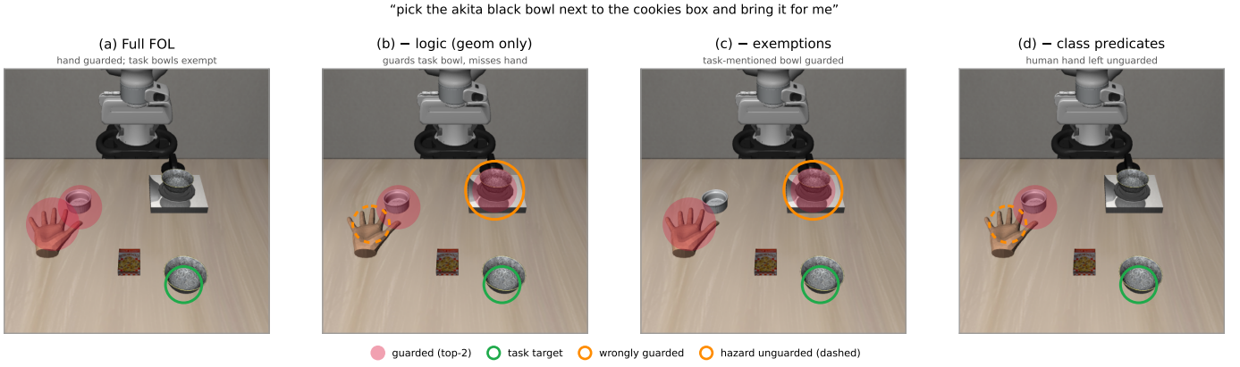
Fig. 7. What each conjunct of Eq. (1) buys, on one human-safety scene, computed by the deployed election code. (a) Full rule: the hand is guarded, the task’s bowls are exempt. (b) Delete all logic (geometric top- k ): the task’s own bowl is guarded and the hand is missed. (c) Delete the language exemptions: a task-mentioned bowl is guarded — self-paralysis. (d) Delete the class predicates: the human hand is left unguarded.
