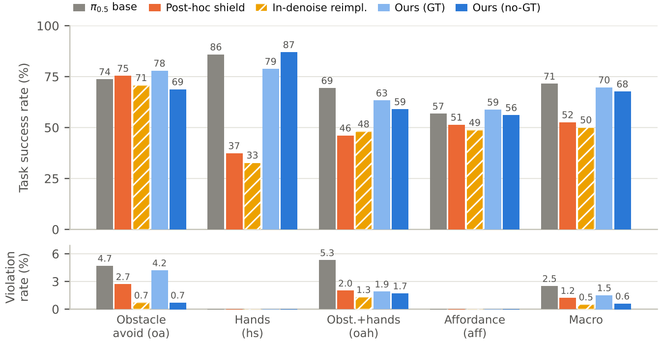
Fig. 5. The LIBERO-Safety five-arm board (Table IV) as task success (top) over benchmark violation rate (bottom). Both dedicated shields collapse the human-safety suite (37.3/32.7 vs. baseline 85.8) while our no-GT stack holds it at baseline — safety by freezing versus safety while moving — and cuts violations to 0.6% macro vs. the baseline’s 2.5%.
