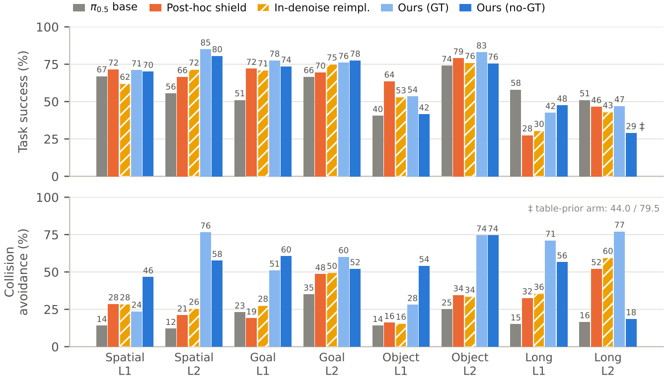
Fig. 4. The SafeLIBERO five-arm board (Table III) as task success (top) over collision avoidance (bottom), eight cells. The no-GT column beats both the baseline and the SOTA reimplement on both axes in 4/8 cells; every shield architecture collapses Long-horizon success.
