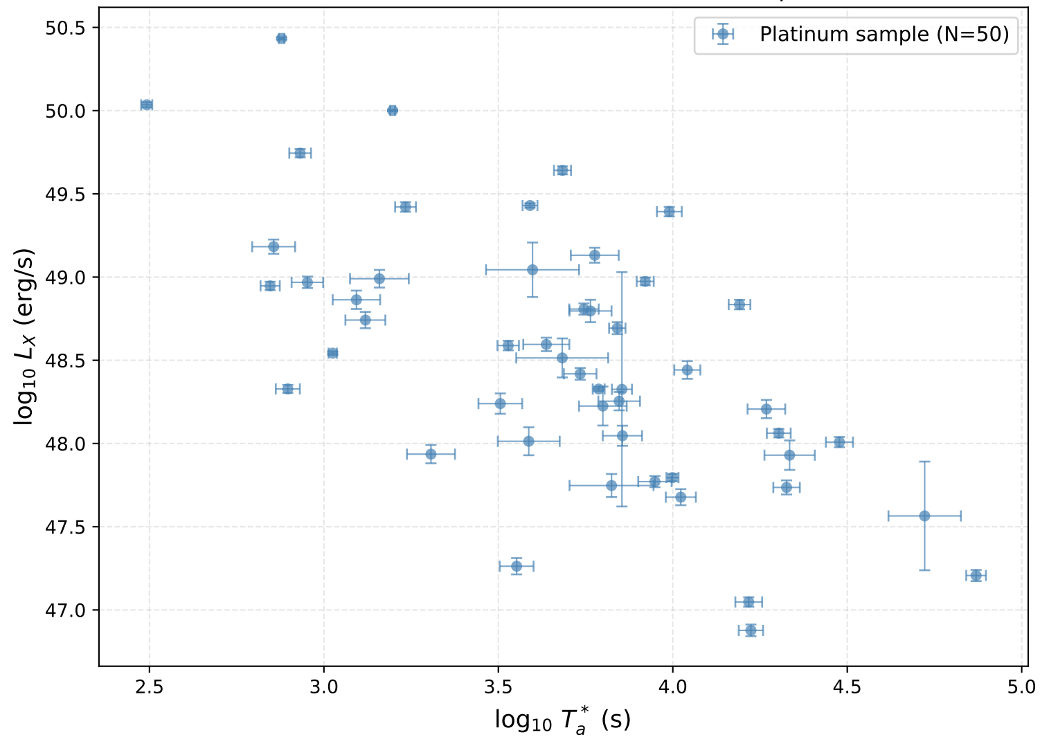
Dainotti Relation — Platinum GRB Sample
