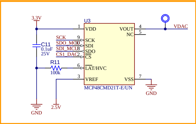
DAC: 12-bit, Single channel, SPI (MSOP-10)
