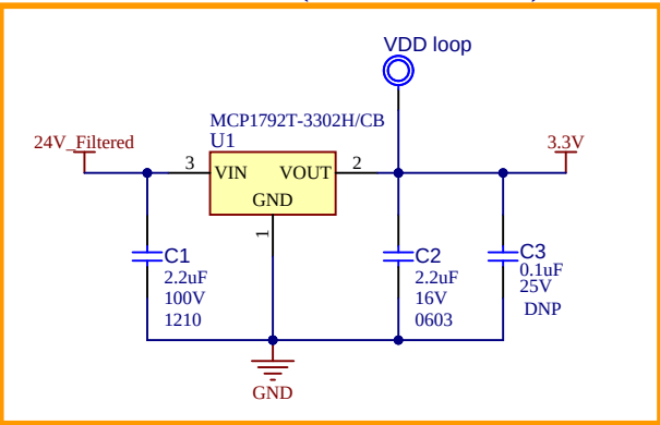
LDO: 3.3V, 100mA (3 lead SOT-23A)
