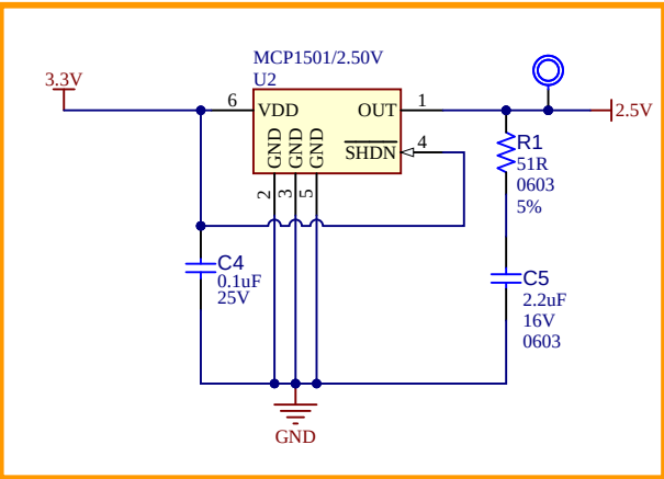
VREF: 2.5V, 50ppm (6 lead SOT-23)
