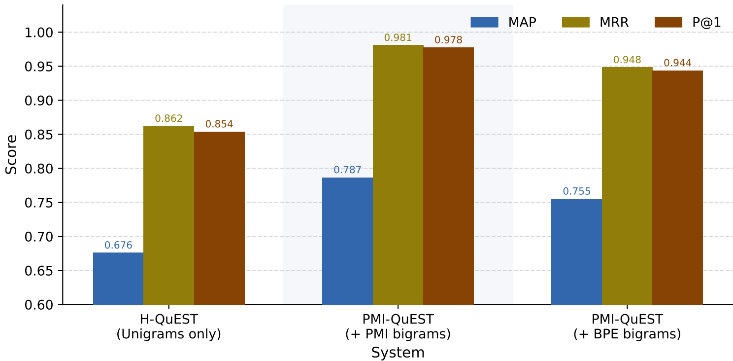
PMI-bigrams vs BPE-bigrams: Ablation on LibriSpeech test-clean (BEST-STD, K=1024, \tau=0.5 , \alpha=1.0 , C=200)
