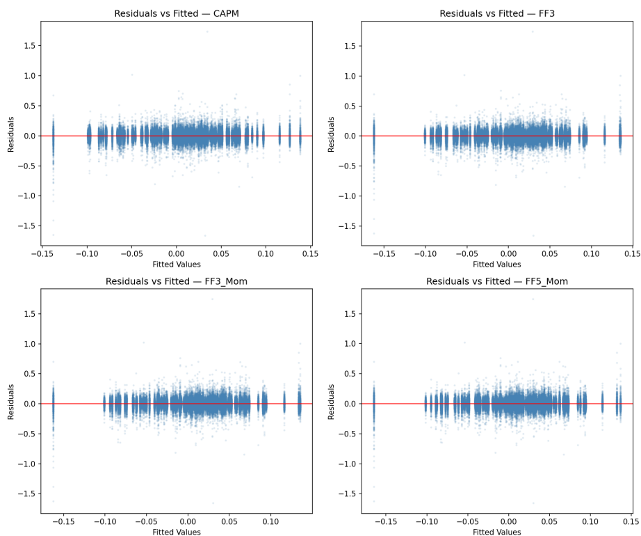
Figure 2: Residual vs Fitted for Fama-French 5 factor+ Momentum
