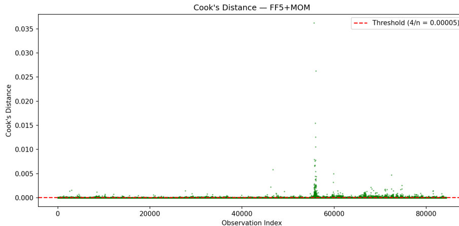
Figure 4: Cook's Distance
