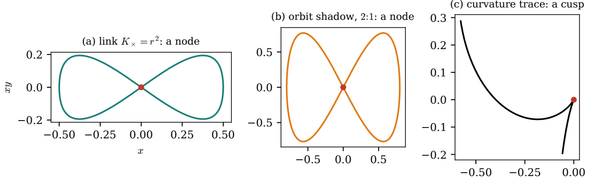
Figure 7: The three curves of Proposition 5.3. (a) The image of the real link K_\times = r^2 ( r = \frac{1}{2} ), projected to the (x, xy) -plane; the node is the double point (0, 0, r) . (b) The shadow of a weighted orbit ( b = 0.8 ). (c) The exceptional principal-curvature trace of the lateral cross-cap P_+ , computed from the exact invariants: an ordinary cusp.
