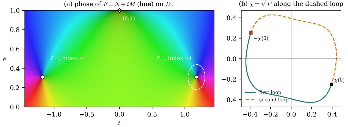
Figure 4: (a) The phase of the observation field F on D_\circ (shown for |t| \leq 1.45 ; brightness increases with |F| ). Every colour meets P_\pm , the dipole of Theorem 4.1. (b) A continuous square root \chi of F along the dashed loop about P_+ : one traversal ends at -\chi(0) , two traversals restore \chi(0) .
