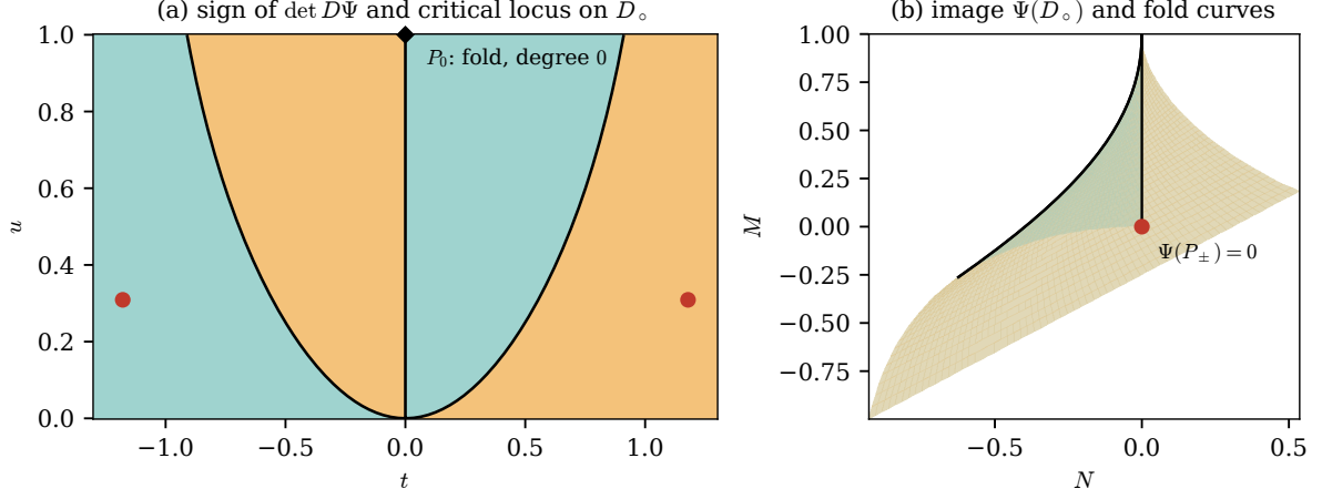
Figure 5: The planar observation map \Psi = (N, M) , shown for |t| \leq 1.3 . (a) The sign of \det D\Psi and the critical locus: the symmetry segment t = 0 and the rational branch through (0, 0) . (b) The image; overlapping sheets (darker) are the two-preimage side of each fold, and the critical values are drawn in black. Both lateral cross-caps map to the origin.
