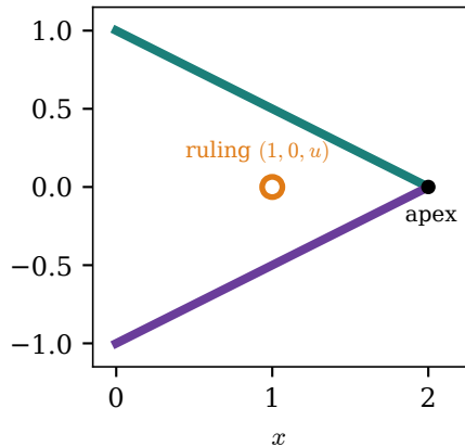
(c) two lines in the plane z = 0
