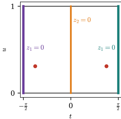
(a) |z_1|^2 = \cos t on D
