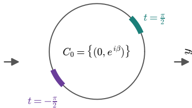
(b) one circle of edge states
