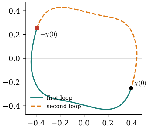
(b) \chi = \sqrt{F} along the dashed loop
