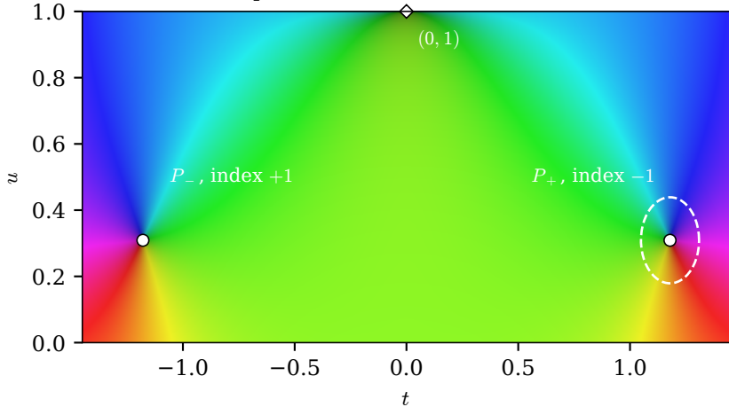
(a) phase of F = N + iM (hue) on D_\circ
