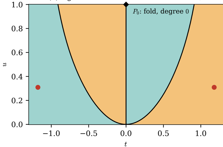
(a) sign of \det D\Psi and critical locus on D_\circ .
