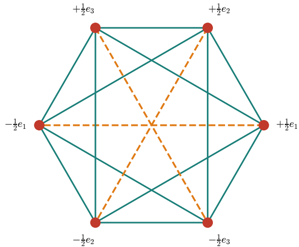
(b) P_{\circ} (solid, octahedron) and P_{\perp} (dashed)
