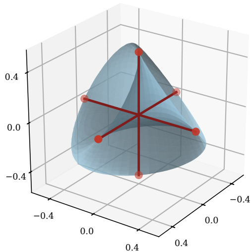
(a) Roman surface: double segments, six cross-caps
