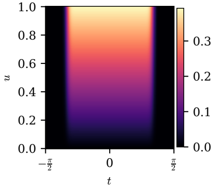
(b) \arg z_1 = \theta \Lambda(c) u
