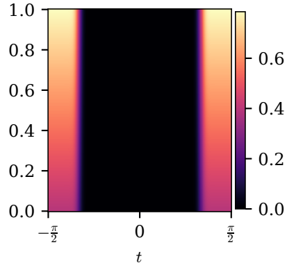
(c) \arg z_2 - \nu\pi = \theta(1 - \Lambda)(1 + u)
