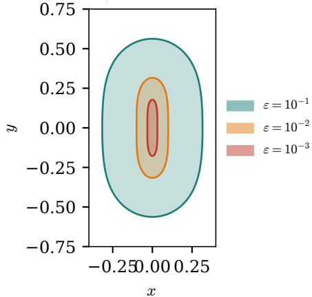
(a) \{K_{\times} \leq \varepsilon\} : width \sqrt{\varepsilon} , height \varepsilon^{1/4}
