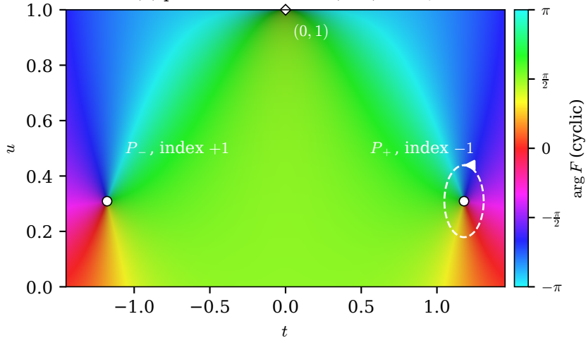
(a) phase of F = N + iM (hue) on D_\circ
