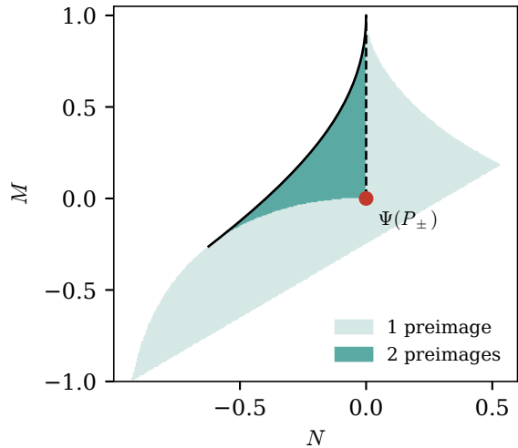
(b) image of 0 \leq t \leq 1.3 , with multiplicity
