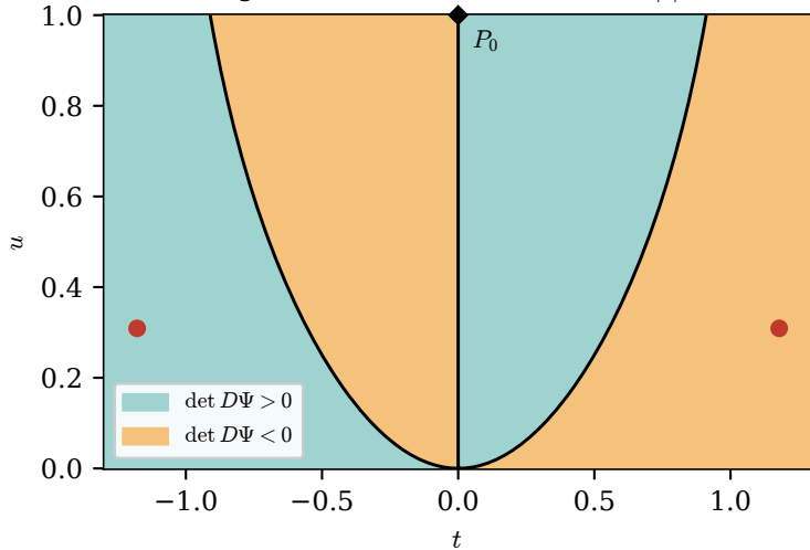
(a) sign of \det D\Psi and critical locus, |t| \leq 1.3
