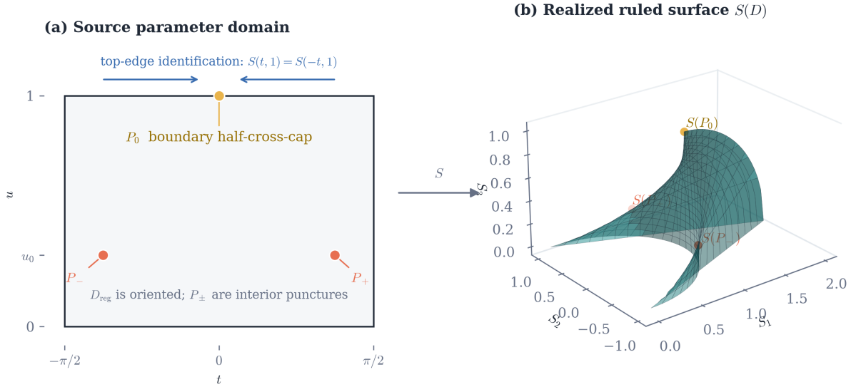
Figure 2: Source and realization atlas for the immersion (1). The two lateral interior points P_{\pm} are the rank-loss cross-caps, while P_0 is the boundary half-cross-cap. The top-edge relation S(t, 1) = S(-t, 1) has the fixed point P_0 ; it is not a free gluing that makes the source non-orientable. The right panel shows the corresponding realized ruled surface.
