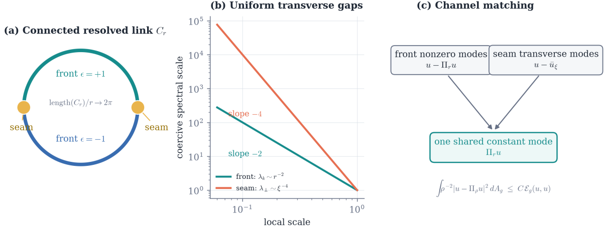
Figure 8: Front–seam decomposition near an interior cross-cap. The two front charts meet through seam charts to give one connected link. Their respective normal scales are r^{-2} and \xi^{-4} ; the uniform estimates leave exactly one matched constant channel and no seam-localized zero mode (Proposition 8.12).
