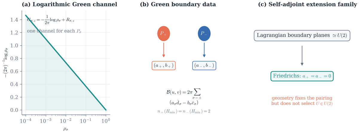
Figure 9: Local Green data and the extension classification at the two interior cross-caps. Each puncture has the logarithmic channel a_\sigma \log \varrho_\sigma + b_\sigma + o(1) and the displayed symplectic Green pairing. Maximal Lagrangian boundary conditions form a U(2) family; the fixed-boundary Friedrichs member sets a_+ = a_- = 0 (Proposition 8.13).
