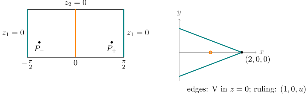
Figure 1: Under the original powers, z_1 vanishes on both edges and z_2 on the polar ruling. The edges map to a V in the plane z = 0 , which no analytic image of C_0 can contain. The ruling maps onto a segment over (1, 0) , on a line skew to both legs.
