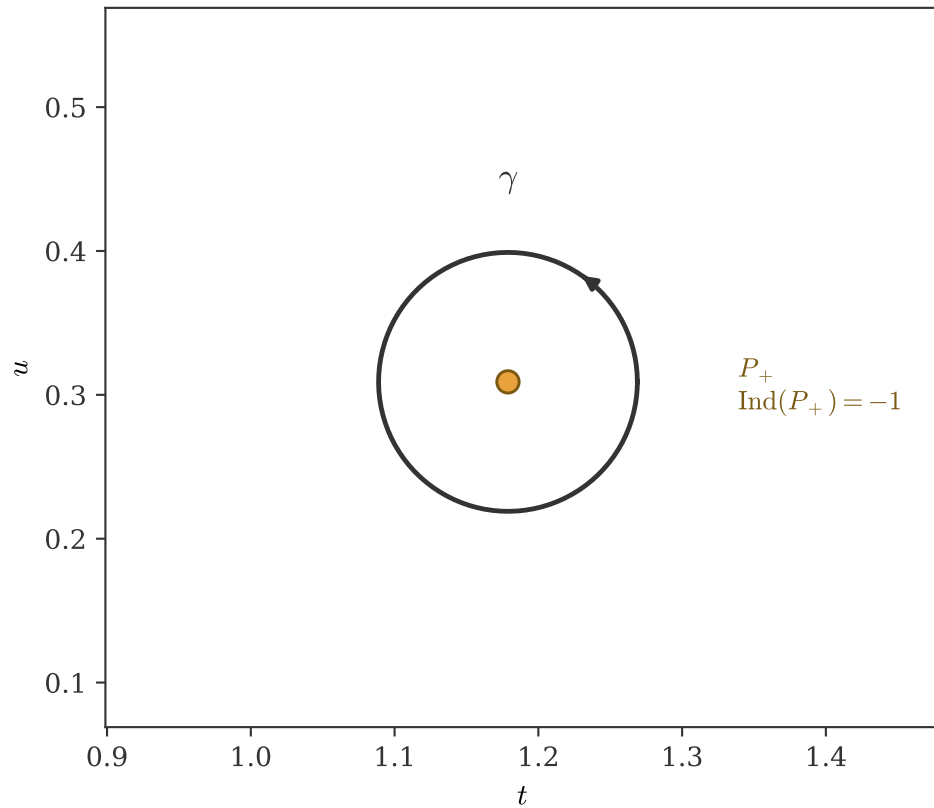
Loop \gamma encircling P_+ in parameter space
