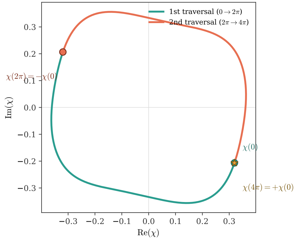
Trajectory of \chi = \sqrt{F} : half turn per traversal of \gamma
