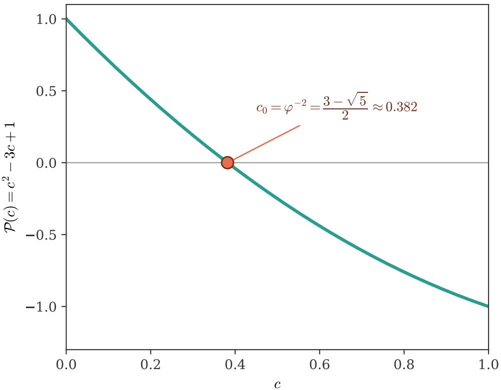
Governing invariant \mathcal{P}(c) (Proposition 6.1)
