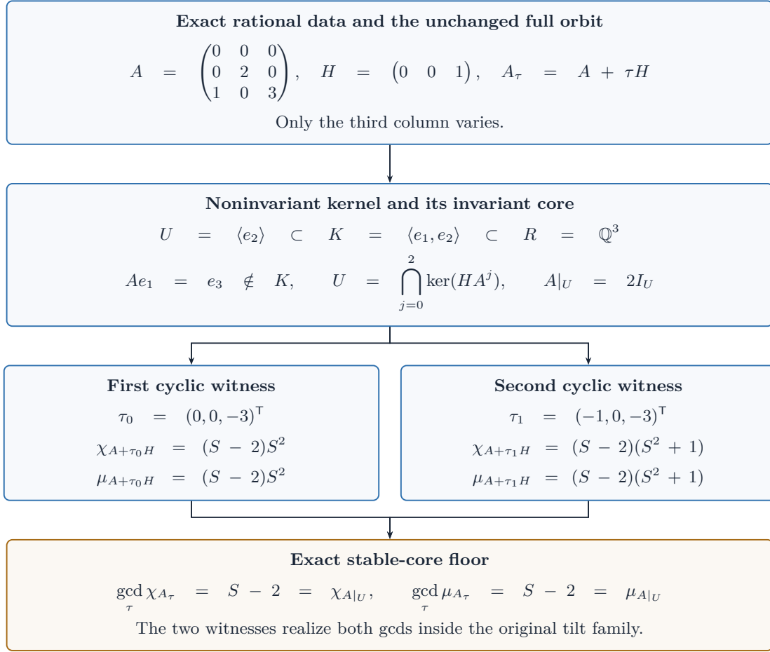
FIGURE 8. An exact noninvariant-normalization floor. The matrices for \tau_0 and \tau_1 are cyclic, so the displayed characteristic and minimal polynomials coincide for each witness. Their gcd is S-2 , precisely the polynomial of the invariant core \mathbb{Q}e_2 . All variations remain confined to the third column.
