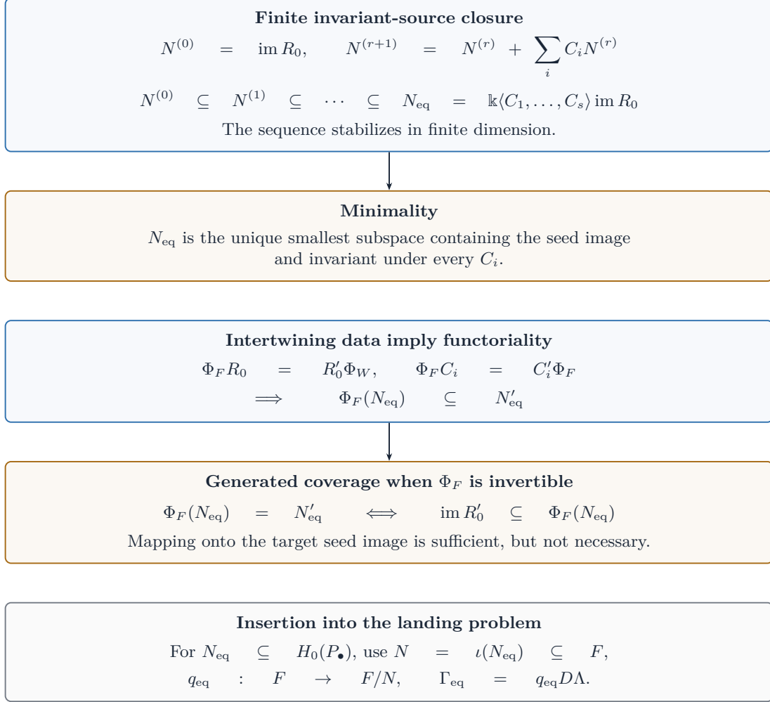
FIGURE 5. Generating the normalized source. Intertwining maps preserve the generated source. For an invertible ambient comparison, equality is equivalent to coverage of the target seeds by the generated image; surjectivity onto the target seed image itself is not necessary. The last panel specializes to the relation module on H_0 and its supplied embedding into F .
