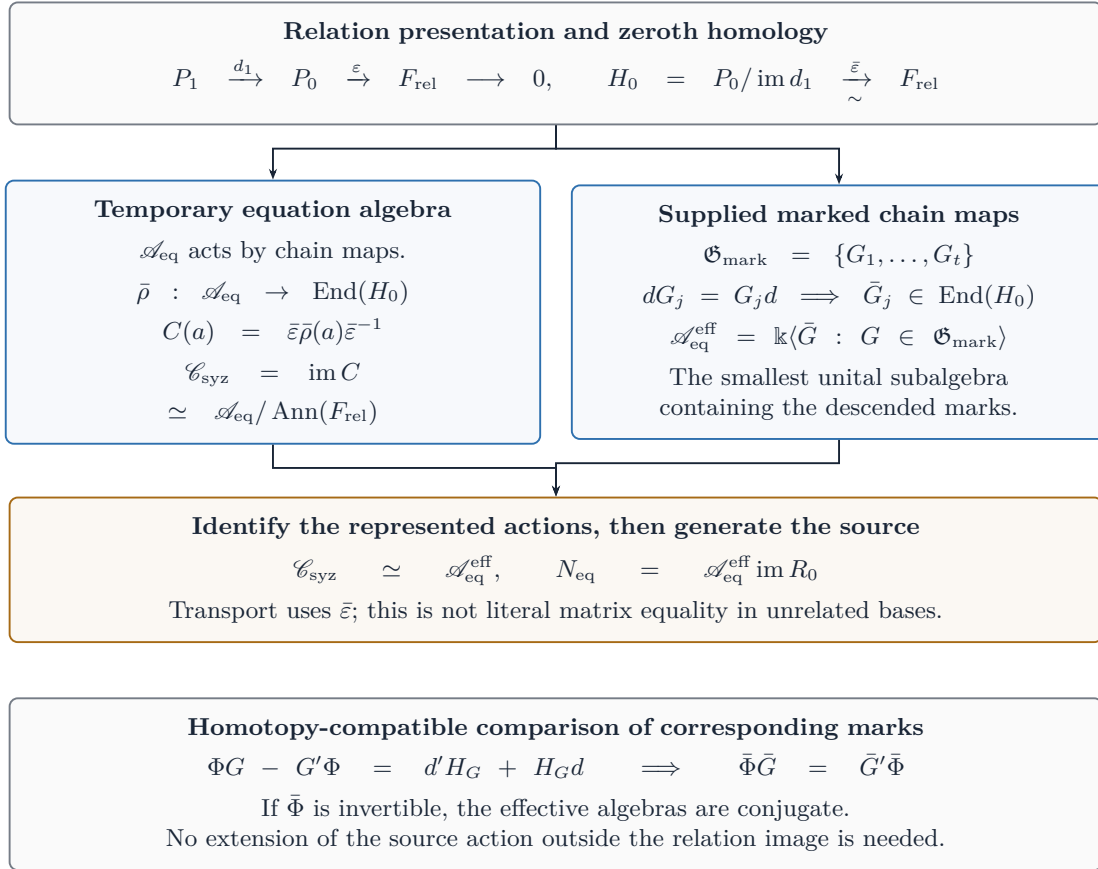
FIGURE 6. From syzygies to the effective equation algebra. The two represented algebras are identified after transporting the same action through the presentation isomorphism. Conjugacy under a homotopy-compatible comparison requires an isomorphism on H_0 , as in Proposition 6.2. No ambient extension outside the relation image is needed.
