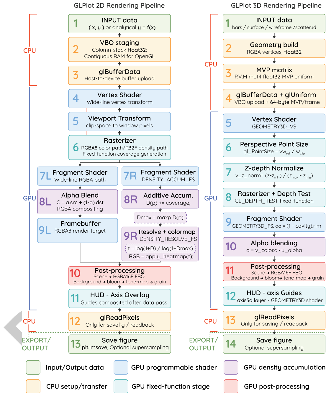
Figure 1: GLPlot's 2D and 3D rendering pipelines, from CPU-side data staging through GPU shading, blending, and post-processing to optional export.
