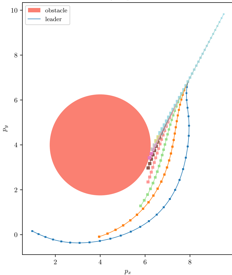
9-vehicle unicycle platoon reach tube
