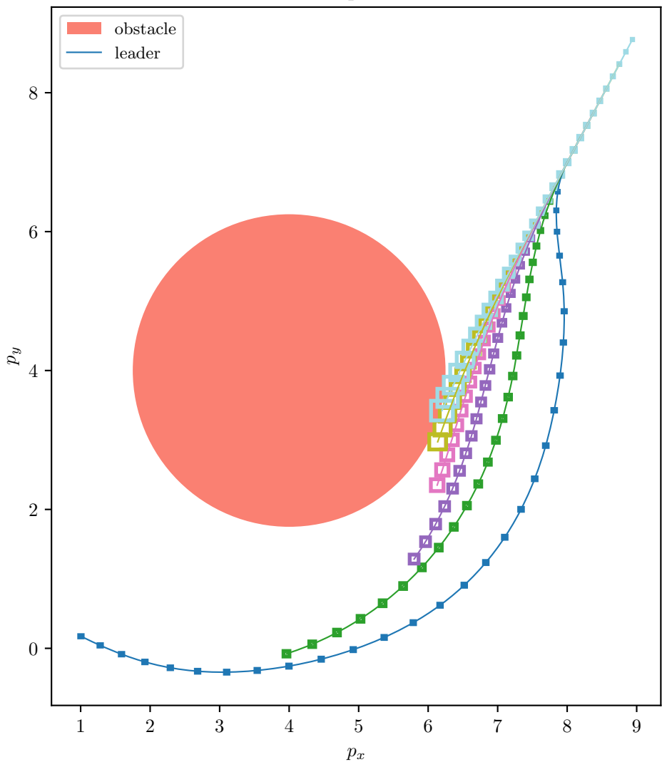
6-vehicle Dubins platoon reach tube
